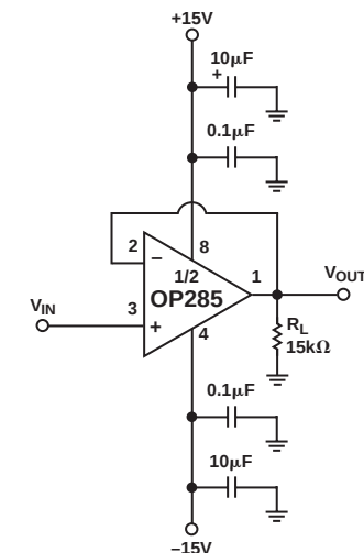
Figure 8. Unity Gain Follower
