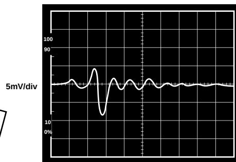
Figure 7. AD9712B/AD9713B Glitch Impulse
