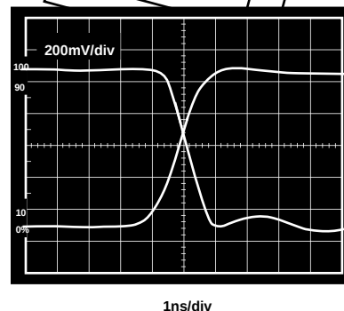
Figure 8. Rise and Fall Characteristics
