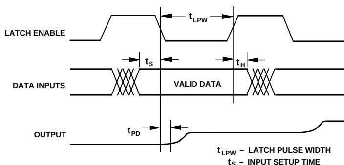
Timing Diagram
