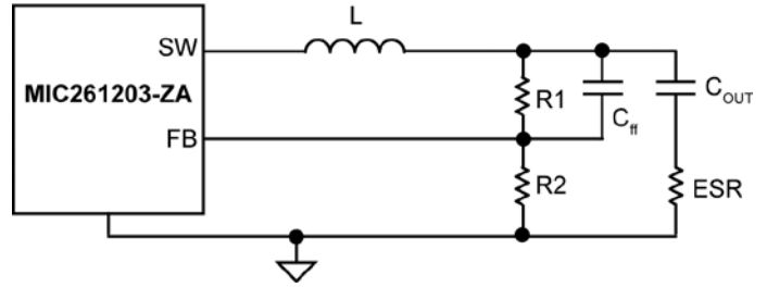
Figure 5. Inadequate Ripple at FB
