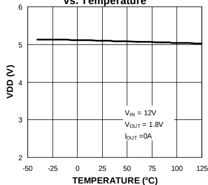
V_{DD} vs. Temperature
