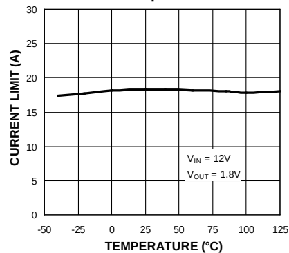
Current Limit vs. Temperature
