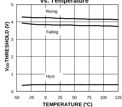
V_{DD} UVLO Threshold vs. Temperature
