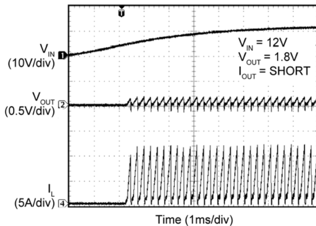
Short Circuit
