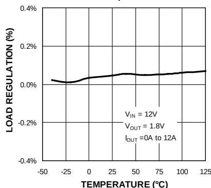
Load Regulation vs. Temperature
