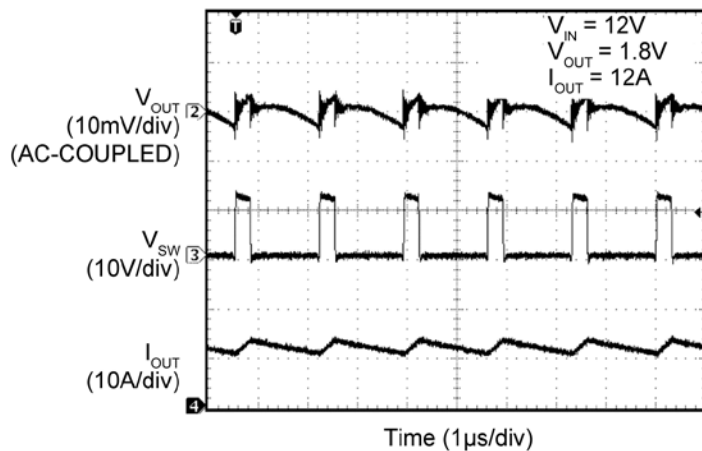
Switching Waveforms
