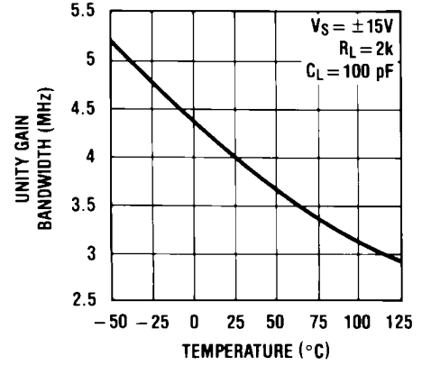
Gain Bandwidth
