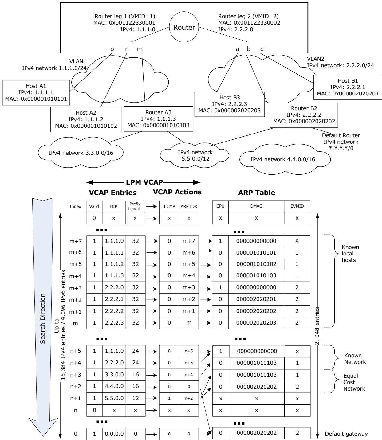
FIGURE 2-25: IP UNICAST ROUTING EXAMPLE
