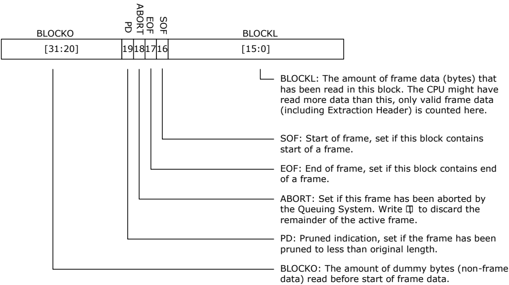
FIGURE 3-13: EXTRACTION STATUS WORD ENCODING
