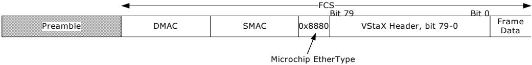
FIGURE 2-4: FRAME WITH VSTAX HEADER
