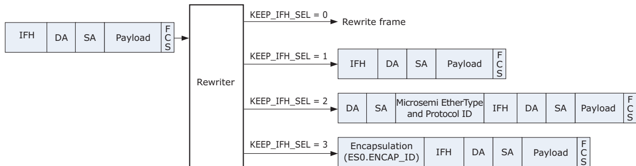
FIGURE 2-101: SUPPORTED KEEP_IFH_SEL FORMATS
