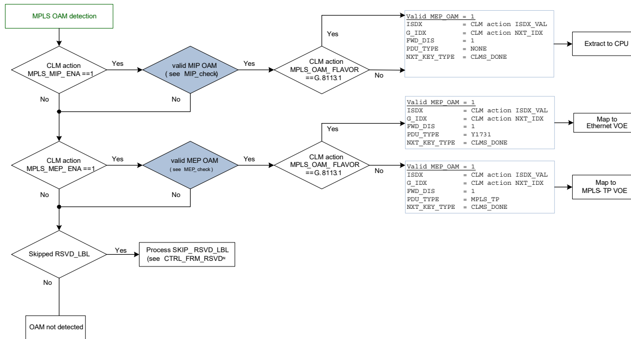
FIGURE 2-17: MPLS OAM DETECTION
