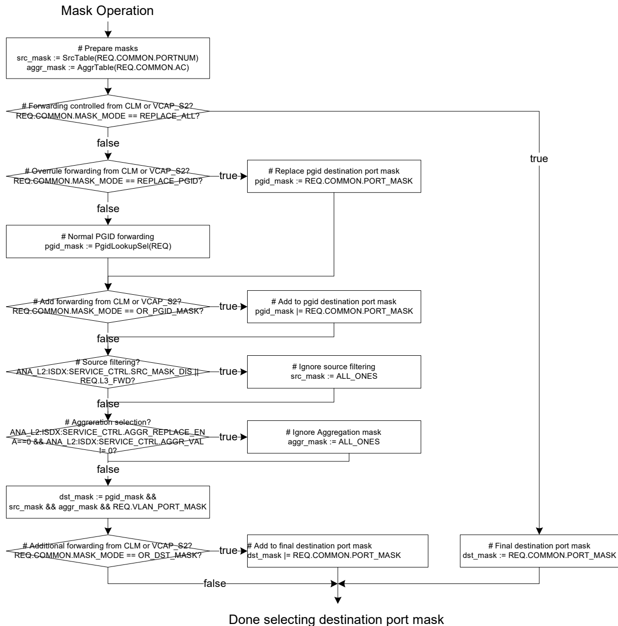
FIGURE 2-34: PORT MASK OPERATION
