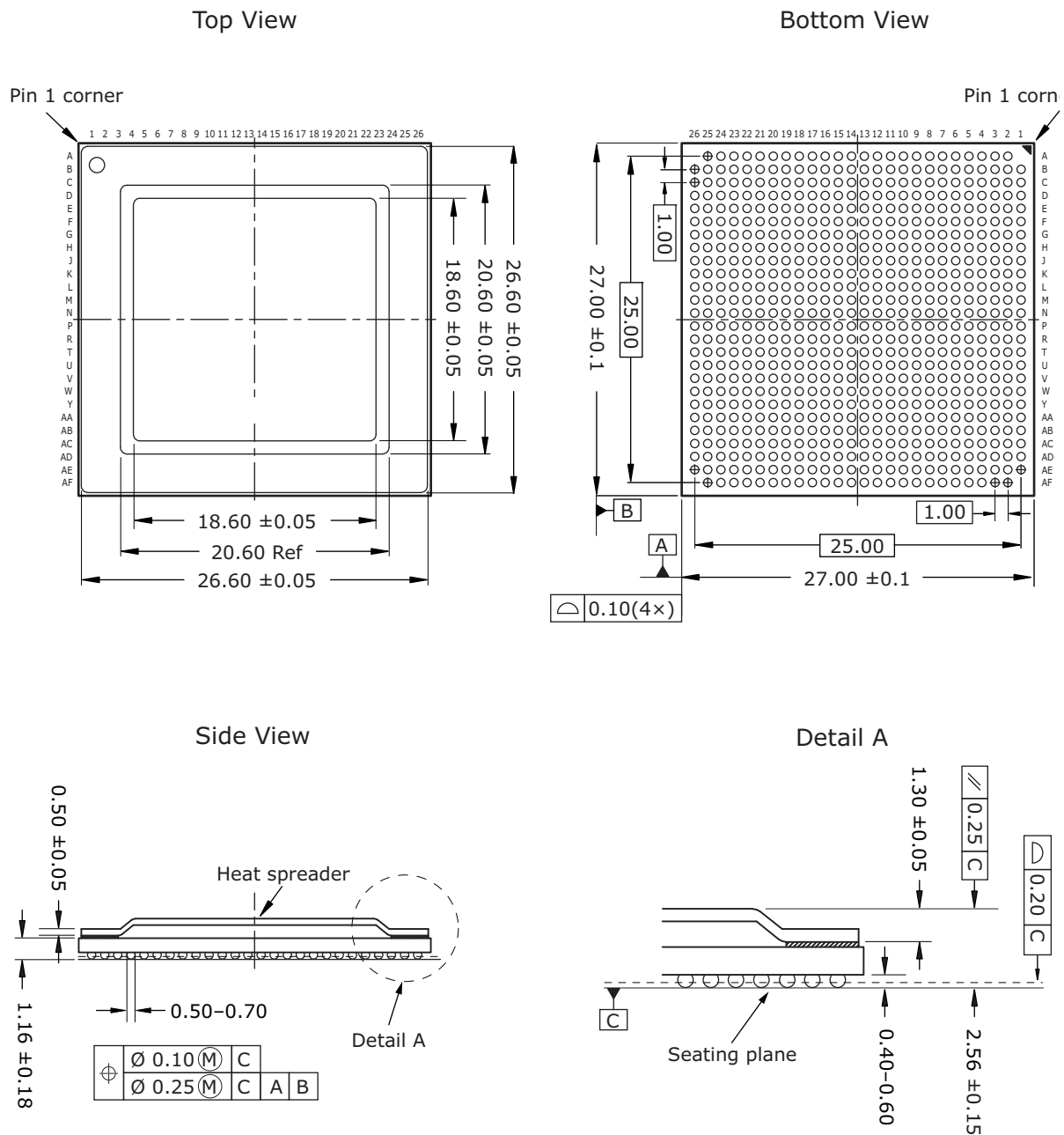
FIGURE 11-1: PACKAGE DRAWING
