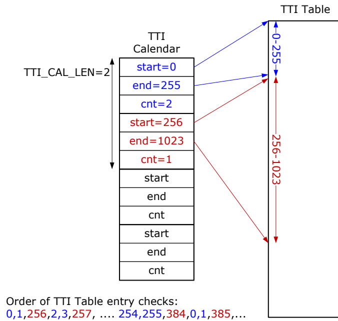
FIGURE 2-93: TTI CALENDAR EXAMPLE
