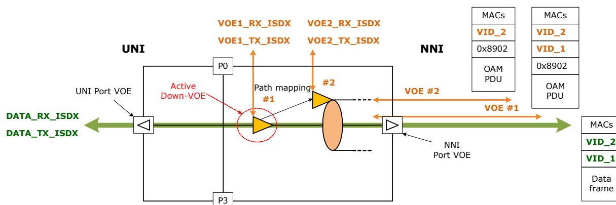
FIGURE 2-50: DOWN-MEP VOE HIERARCHY
