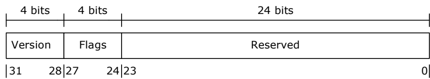
FIGURE 2-107: VRAP HEADER FORMAT
