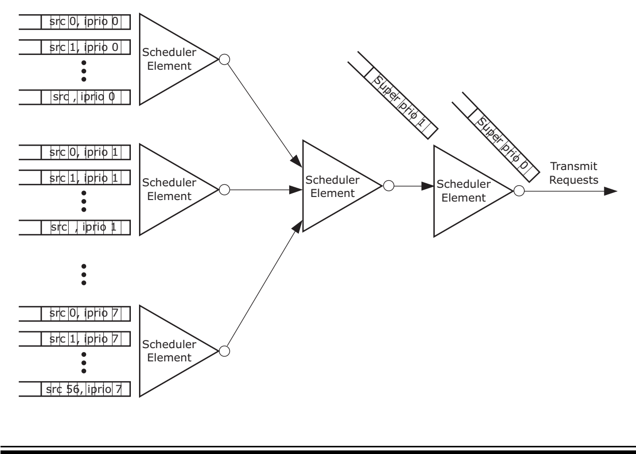
FIGURE 2-78: SCHEDULER HIERARCHY (NORMAL SCHEDULING MODE)
