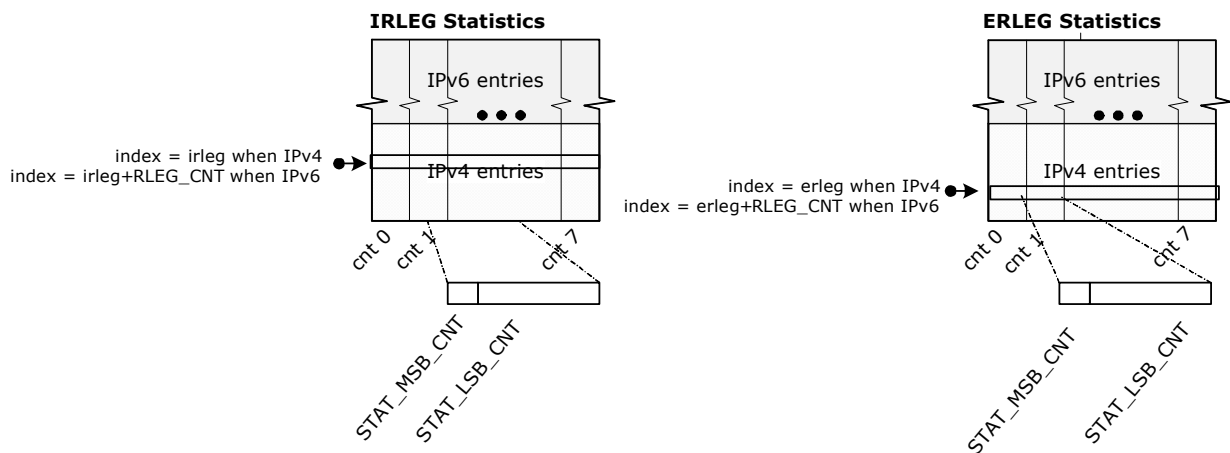
FIGURE 2-43: INGRESS AND EGRESS ROUTING STATISTICS PER ROUTER LEG PER IP VERSION
