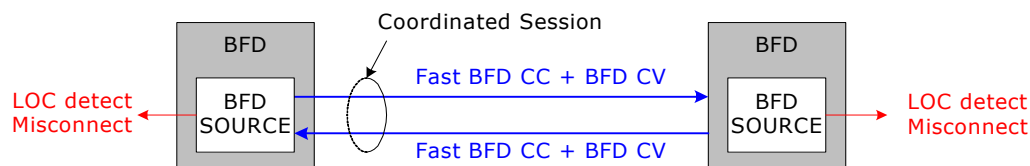
FIGURE 2-68: BFD COORDINATED MODE
