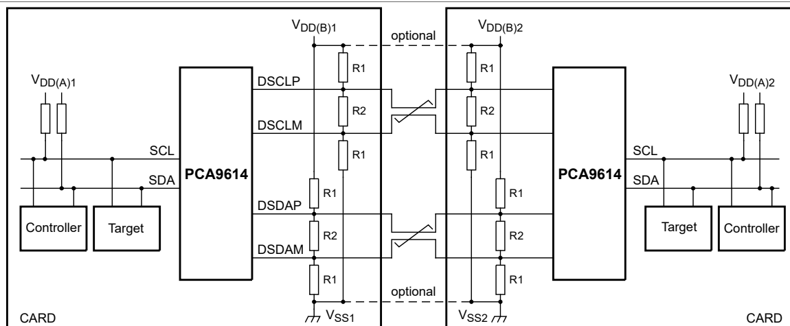
Figure 6. Typical application for PCA9614
