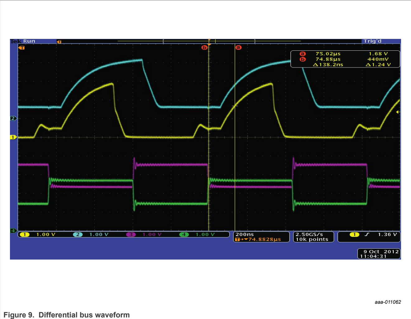
Figure 9. Differential bus waveform
