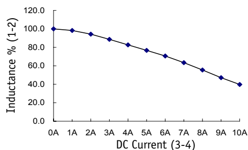
Inductance vs. Current
