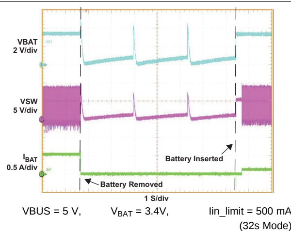
Figure 29. Battery Insertion/Removal
