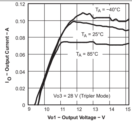
Figure 14. VO3 Maximum Load Current
