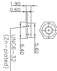
B MOUNTING HOLE 8 PLACE SACLE4:1
