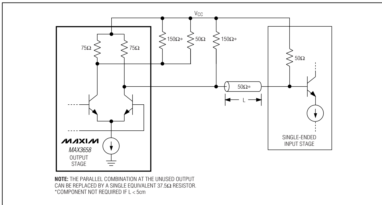
Figure 6b. 50Ω DC-Coupled Single-Ended Output Interface
