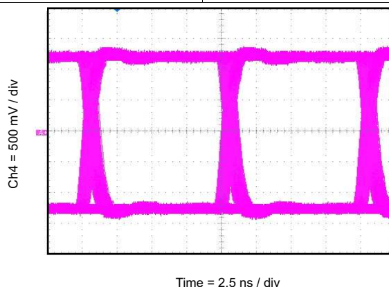
Figure 26. Eye Diagram at 100 Mbps PRBS 2^{16} - 1 , 2.5 V and 25°C
