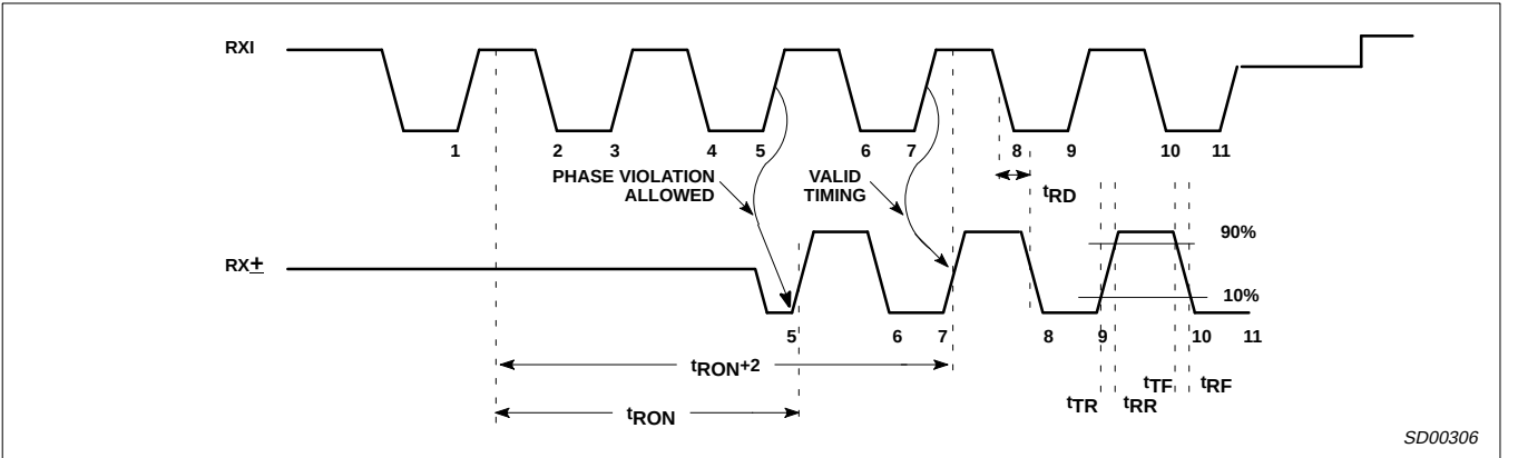
Figure 3. Receiver Timing
