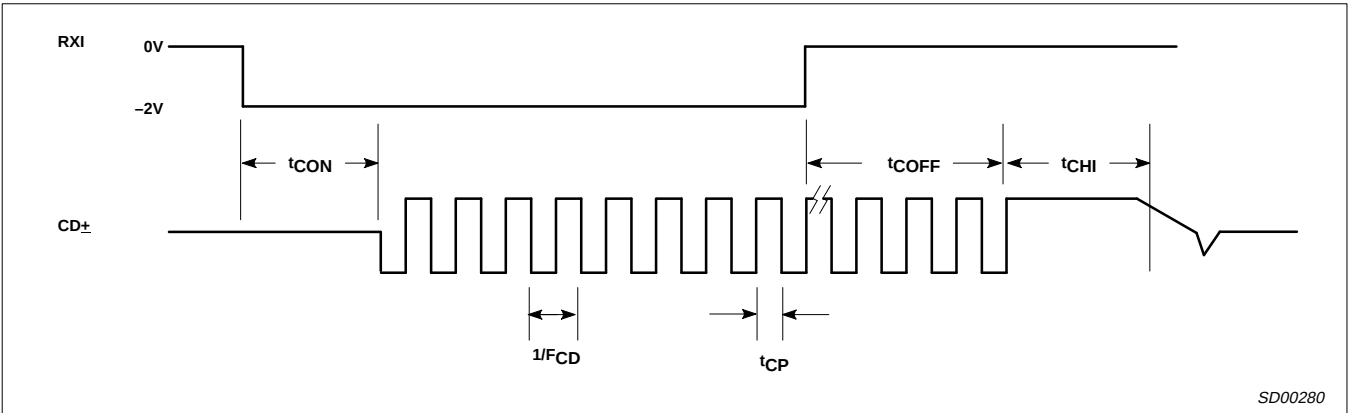
Figure 6. Collision Timing
