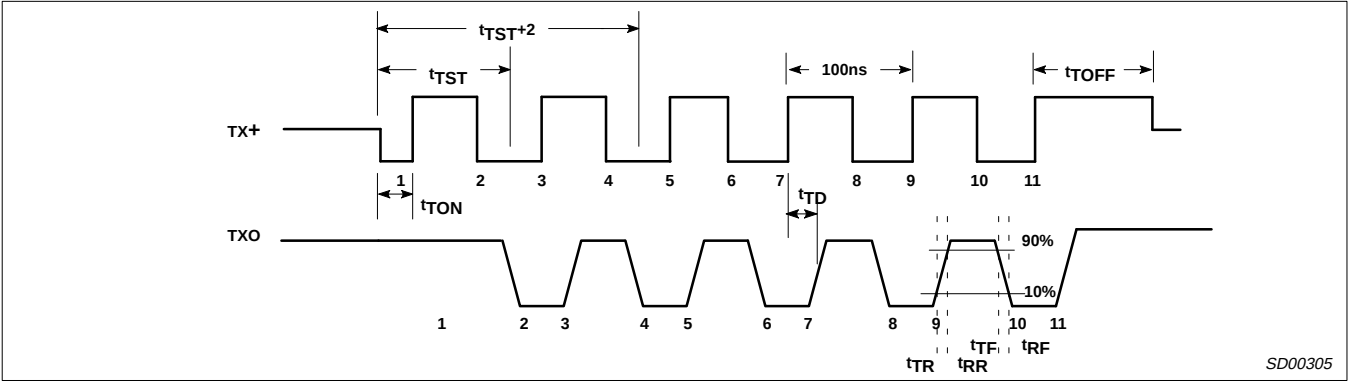
Figure 5. Transmitter Timing
