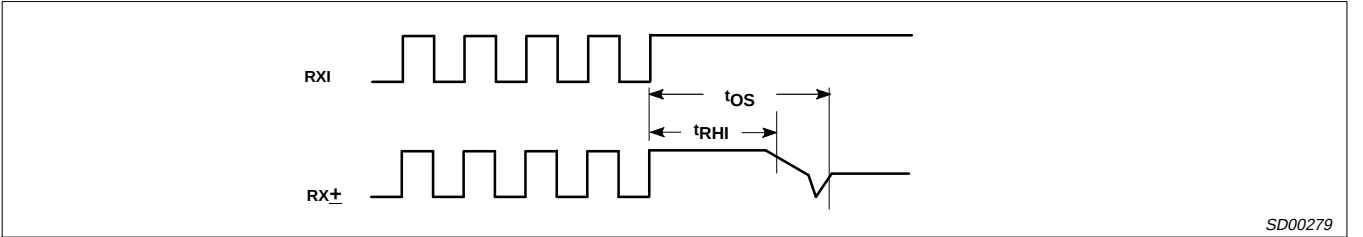
Figure 4. Receiver End-of-Packet Timing
