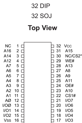
FIGURE 1 – PIN CONFIGURATION
