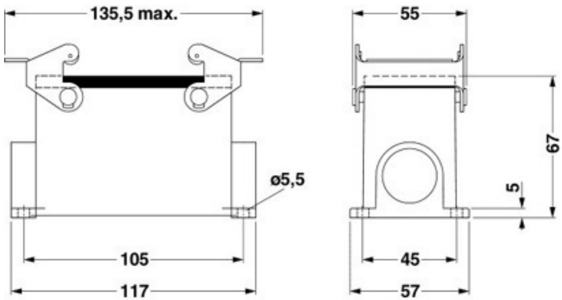
Dimensioned drawing
