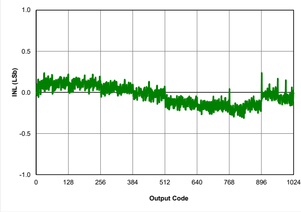
Figure 39-3. ADC, INL, V_{DD} = 3.0V , T_{AD} = 4\mu S , 25°C
