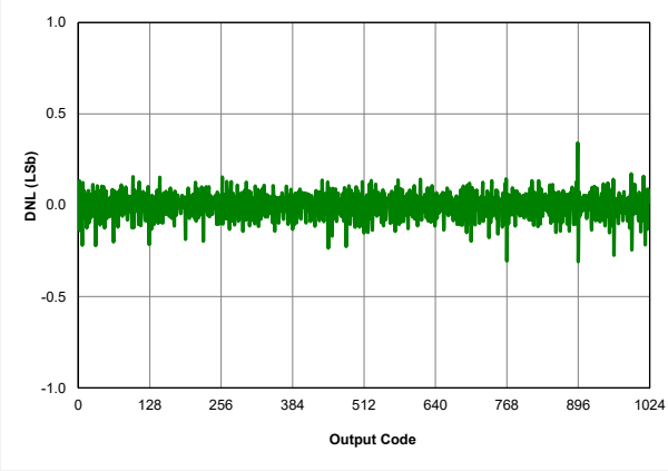
Figure 39-4. ADC, DNL, V_{DD} = 3.0V , T_{AD} = 4\mu S , 25°C
