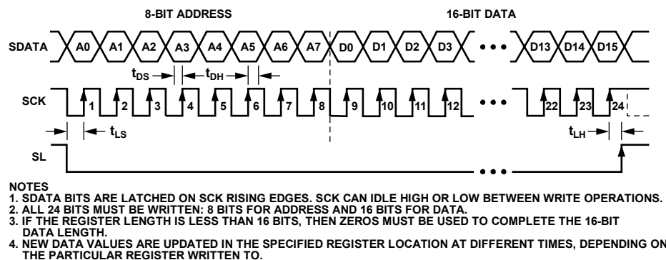
Figure 16. Serial Write Operation
