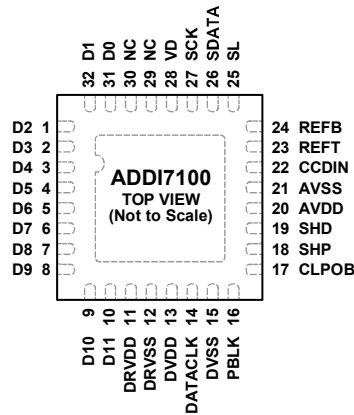
Figure 5. Pin Configuration
