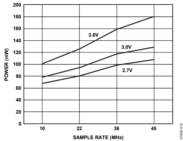
Figure 6. Power vs. Sample Rate
