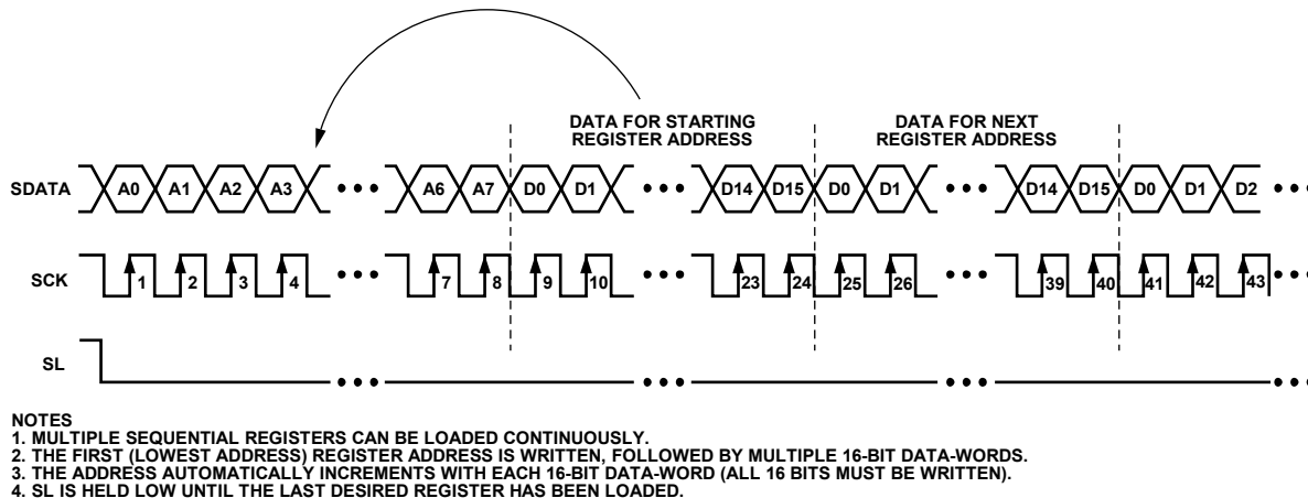
Figure 17. Continuous Serial Write Operation
