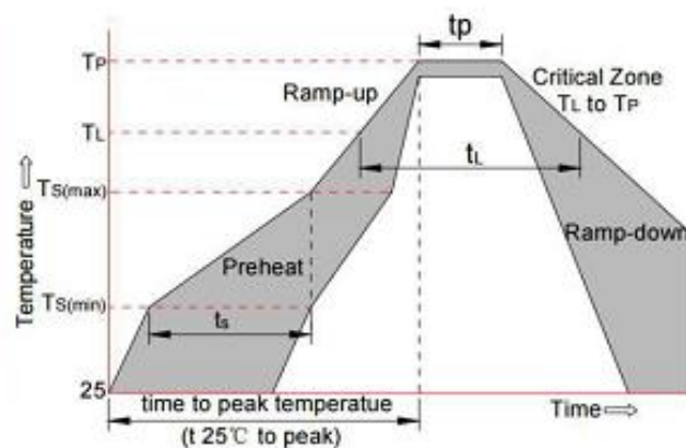
FIG.2: Reflow condition
