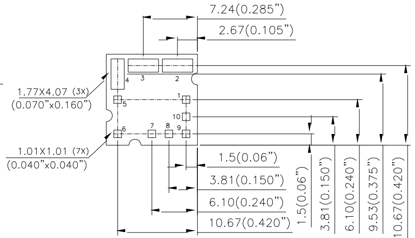
BOTTOM VIEW
