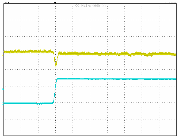
Figure 22: Typical transient response to step load change at 2.5\text{A}/\mu\text{S} from 0% to 100% of I_o , max at 5V_{in} , 1.2V_{out} ( 200\mu\text{S}/\text{div} ) ( C_{out} = 47\mu\text{F} ceramic).top trace: V_{out} , 0.1\text{V}/\text{div} ;bottom trace: I_{out} : 2\text{A}/\text{div} .
