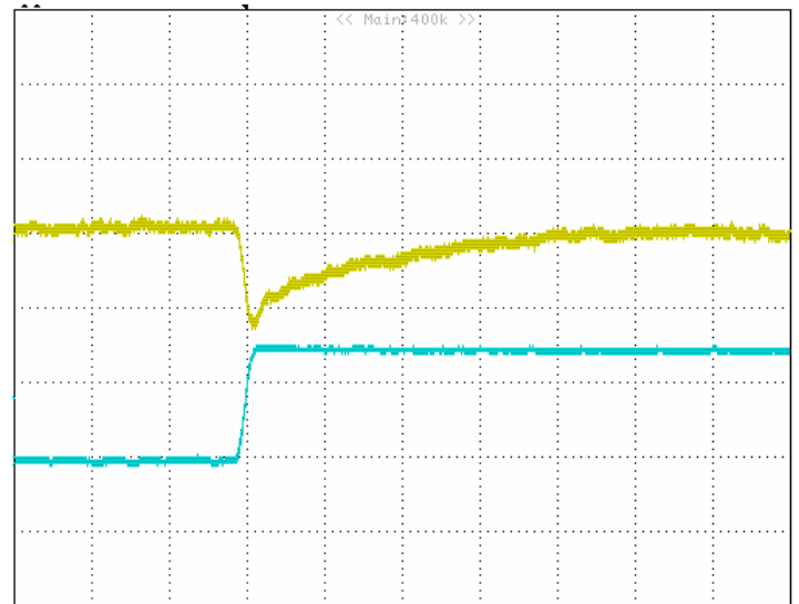
Figure 26: Typical transient response to step load change at 2.5\text{A}/\mu\text{S} from 0% to 100% of I_o , max at 5V_{in} , 3.3V_{out} (200uS/div) ( C_{out} = 47\mu\text{F} ceramic).top trace:Vout,0.1V/div;bottom trace:Iout:2A/div.
