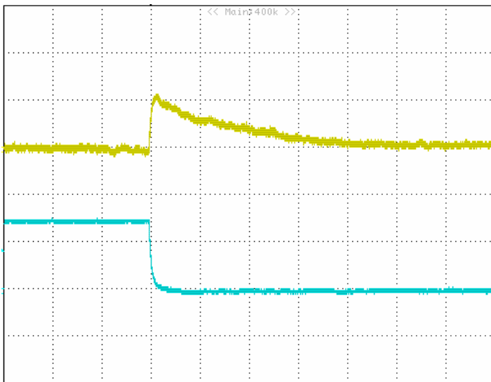
Figure 25: Typical transient response to step load change at 2.5\text{A}/\mu\text{S} from 100% to 0% of I_o , max at 5V_{in} , 3.3V_{out} (200uS/div) ( C_{out} = 47\mu\text{F} ceramic).top trace:Vout,0.1V/div;bottom trace:Iout:2A/div.
