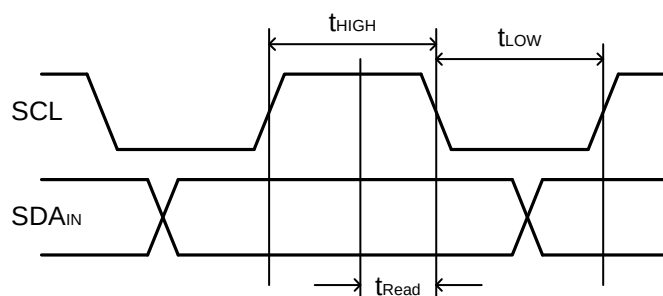
Figure 5-2 : TWSI Read diagram
