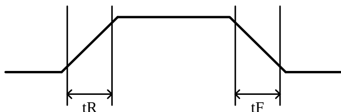
Figure 5-4 : Bus Rising/Falling waveform diagram
