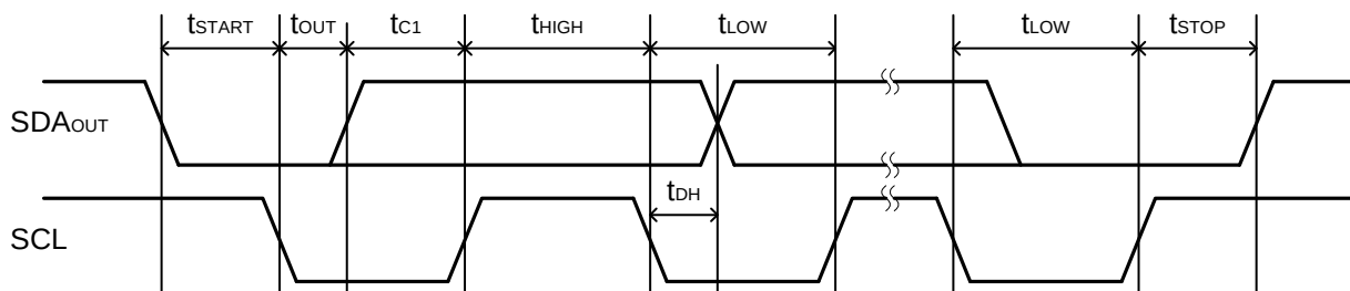
Figure 5-1 : TWSI Start, Stop and Write diagram
