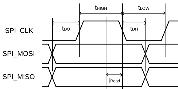
Figure 5-5 : SPI Data Read/Write diagram
