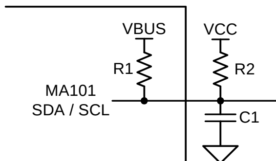
Figure 5-3 : Circuit diagram
