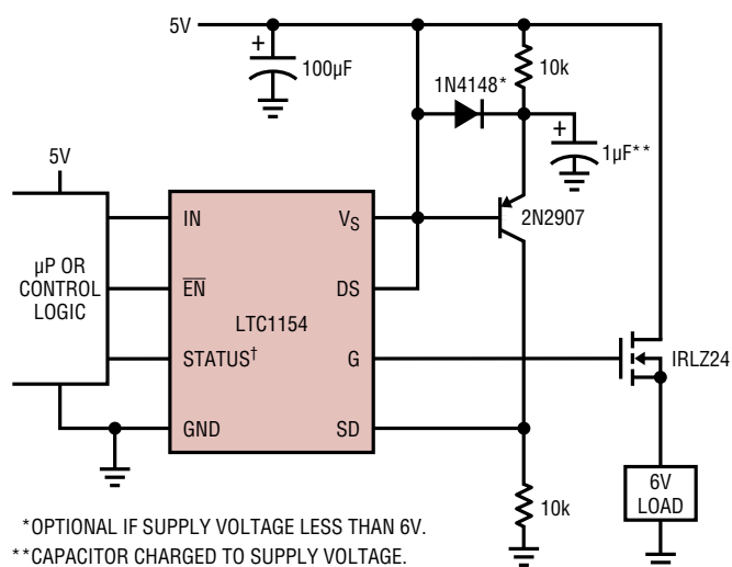
High Side Driver with Undervoltage Shutdown
