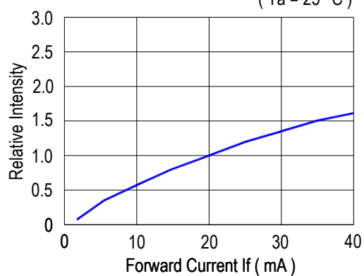
FIG. 2 Relative Intensity vs. Forward Current ( Ta = 25 °C )
