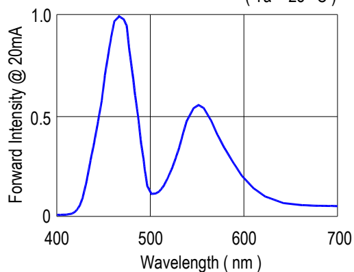
FIG. 5 Relative Intensity vs. Wavelength ( \lambda_p ) ( Ta = 25 °C )
