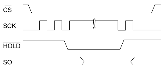
Figure 20. HOLD Operation
