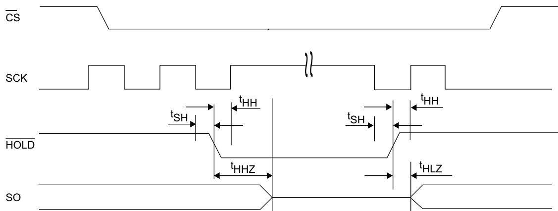
Figure 26. \overline{\text{HOLD}} Timing
