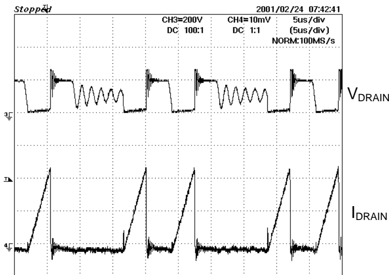
Figure 21. V DRAIN & I DRAIN (200 V & 0.1 A/div) at 3 W Load, 85 V AC Input. (5 µs/div)
