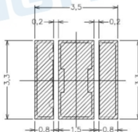
Soldering patterns
