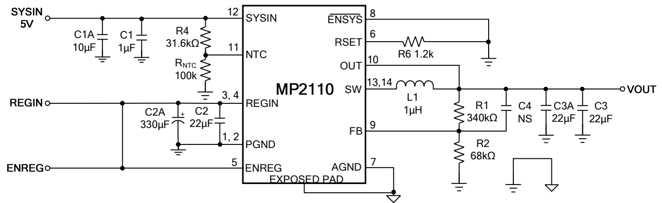
Figure 3: Typical Application, 3.6V Output Voltage
