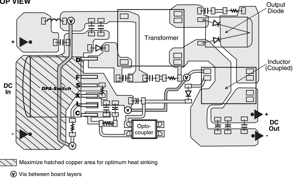
Figure 28. Layout Considerations for DPA-Switch Using R Package.
