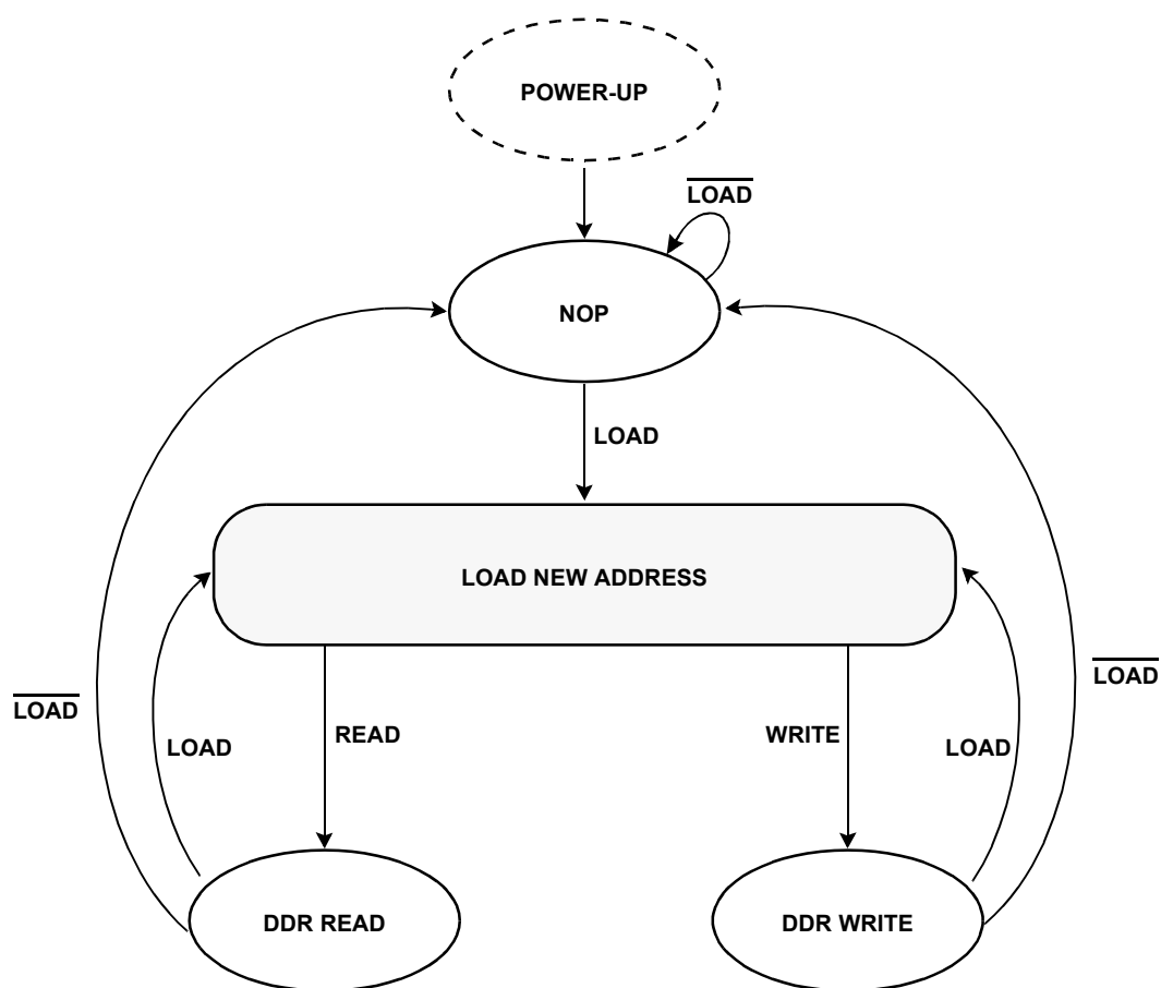
STATE DIAGRAM
