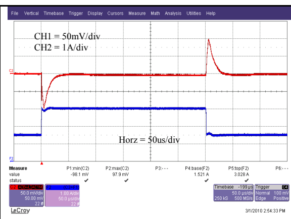
V_o=3.3V Typical output voltage transient response to load step from 50% to 100% of full load with output current slew rate of 10A/uS. (Cext = 2x22uF ceramic capacitor)
