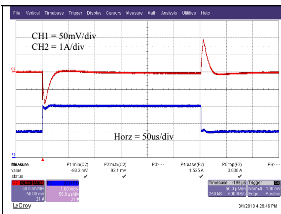
V_o=1.8V Typical output voltage transient response to load step from 50% to 100% of full load with output current slew rate of 10A/uS. (Cext = 2x22uF ceramic capacitor)
