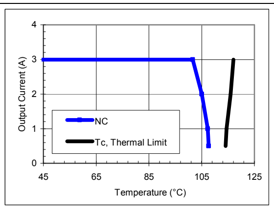
Vo=3.3V, Vin=12V maximum output current vs. ambient temperature at nominal input voltage for natural convection (60lfm) with airflow from pin 7 to pin 3.
