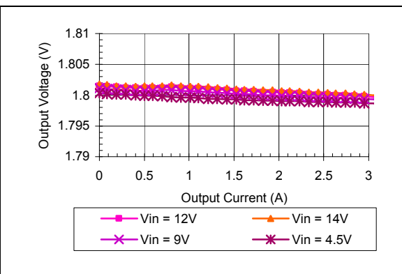
Vo=1.8V Typical load regulation
