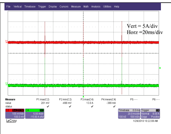
Typical Output Short Circuit Current – CH4, green
