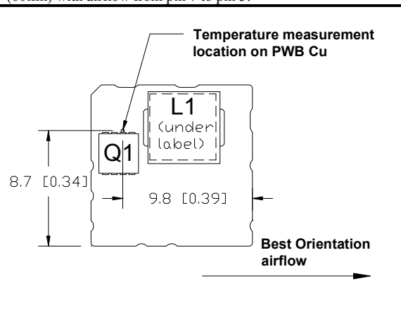
ICF12003A007V thermal measurement location – top view
