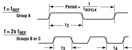
Figure 8. t_{SKEW4}
