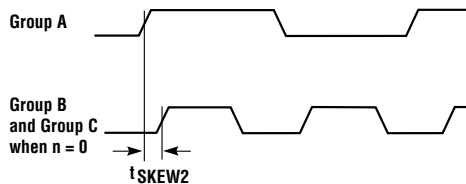
Figure 6. t_{SKEW2}
