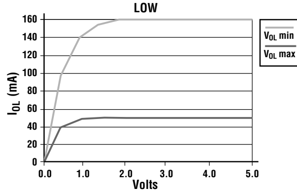
Figure 10. I_{OL} vs. V_{OL}
