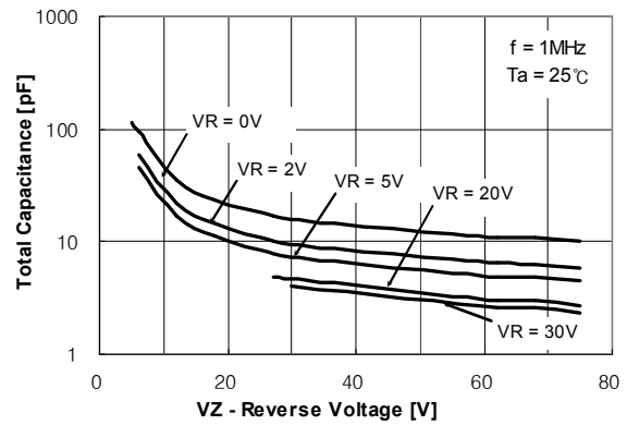
Figure 2. Total Capacitance
