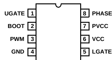
HIP6601ACB, HIP6603ACB (SOIC) HIP6601ECB, HIP6603ECB (EPSONIC) TOP VIEW
