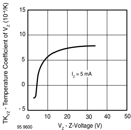
Figure 5. Temperature Coefficient of V_z vs. Z-Voltage
