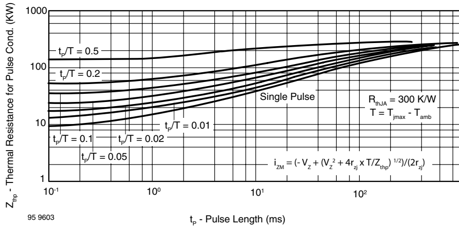
Figure 11. Thermal Response
