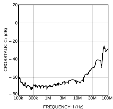
Fig. 3 Interchannel crosstalk
