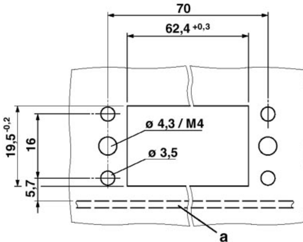
Dimensioned drawing
