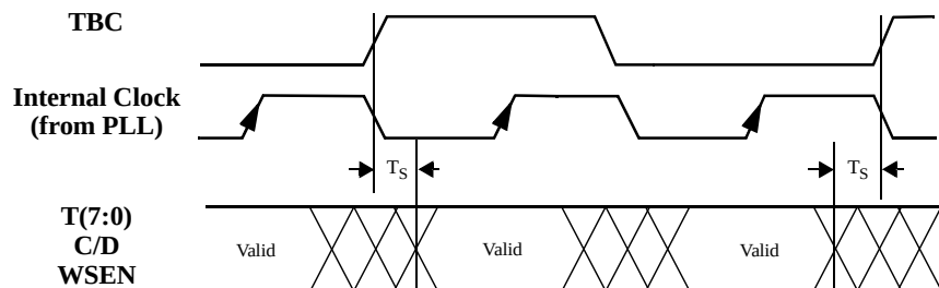
Figure 15: Transmit Input Timing Waveforms with TMODE = 11X (“ASIC-Friendly” Timing)
