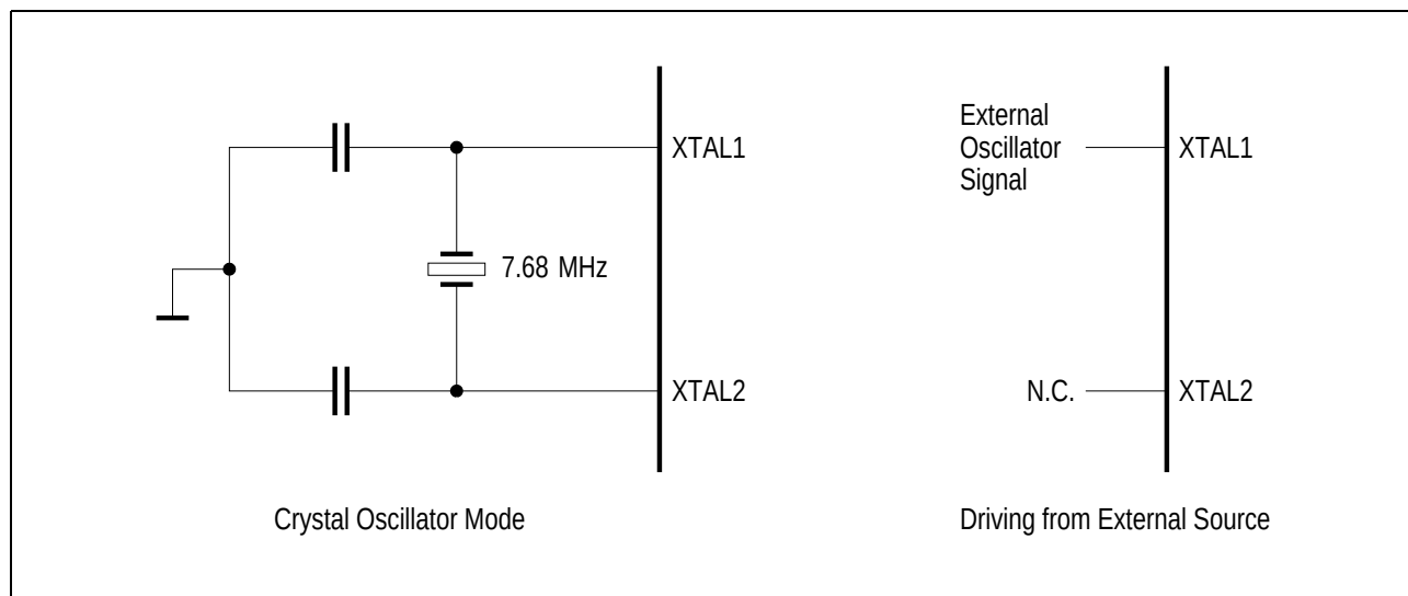
Figure 68 Oscillator Circuits
