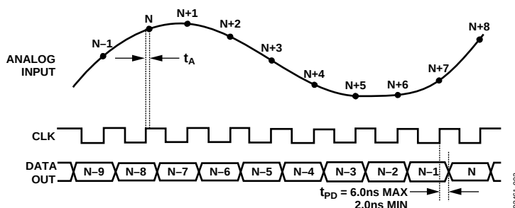
Figure 2. Timing Diagram
