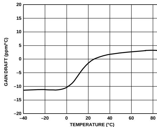
Figure 30. A/D Gain vs. Temperature Using an External Reference
