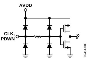
Figure 8. Equivalent Digital Input Circuit
