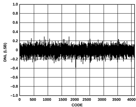
Figure 32. Typical DNL
