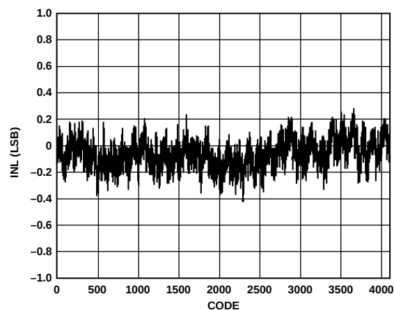
Figure 31. Typical INL
