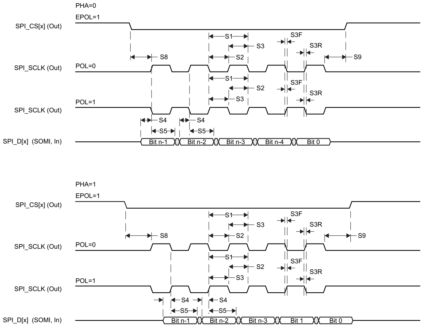
Figure 5-82. SPI Master Mode Receive Timing
