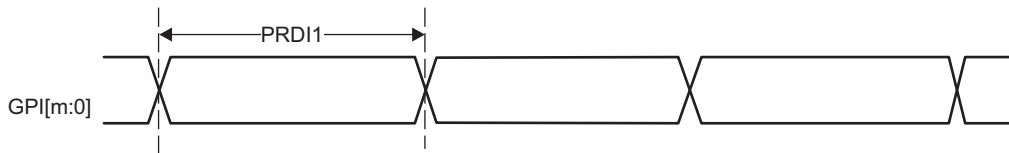
Figure 5-58. PRU-ICSS PRU Direct Input Timing
