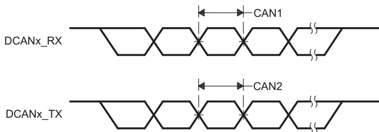
Figure 5-19. DCANx Timings
