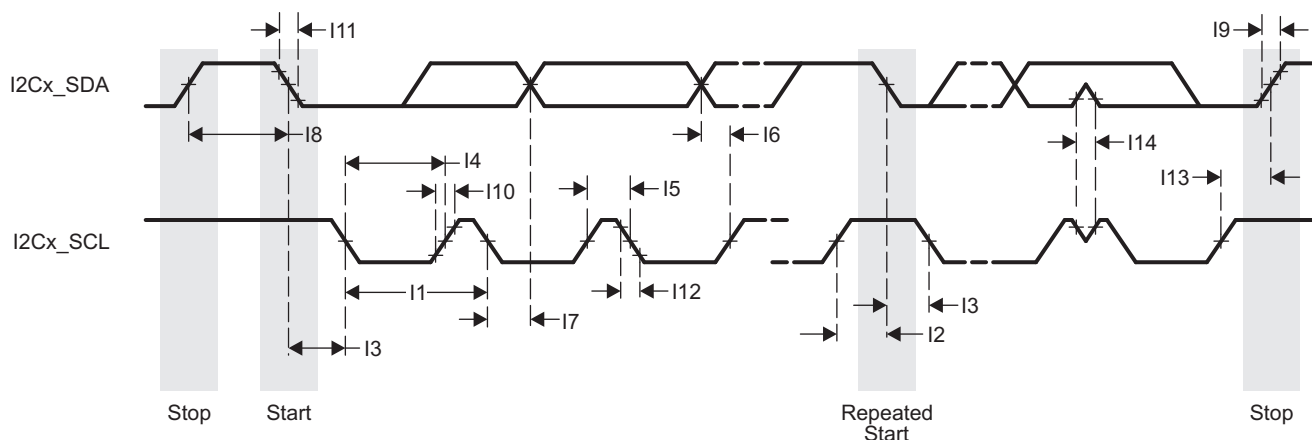
Figure 5-43. I2C Receive Timing (1)
