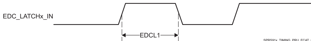
Figure 5-65. PRU-ICSS ECAT LATCHx_IN Timing
