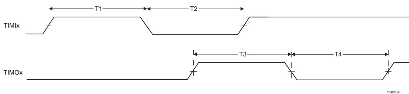
Figure 5-84. Timer Timing
