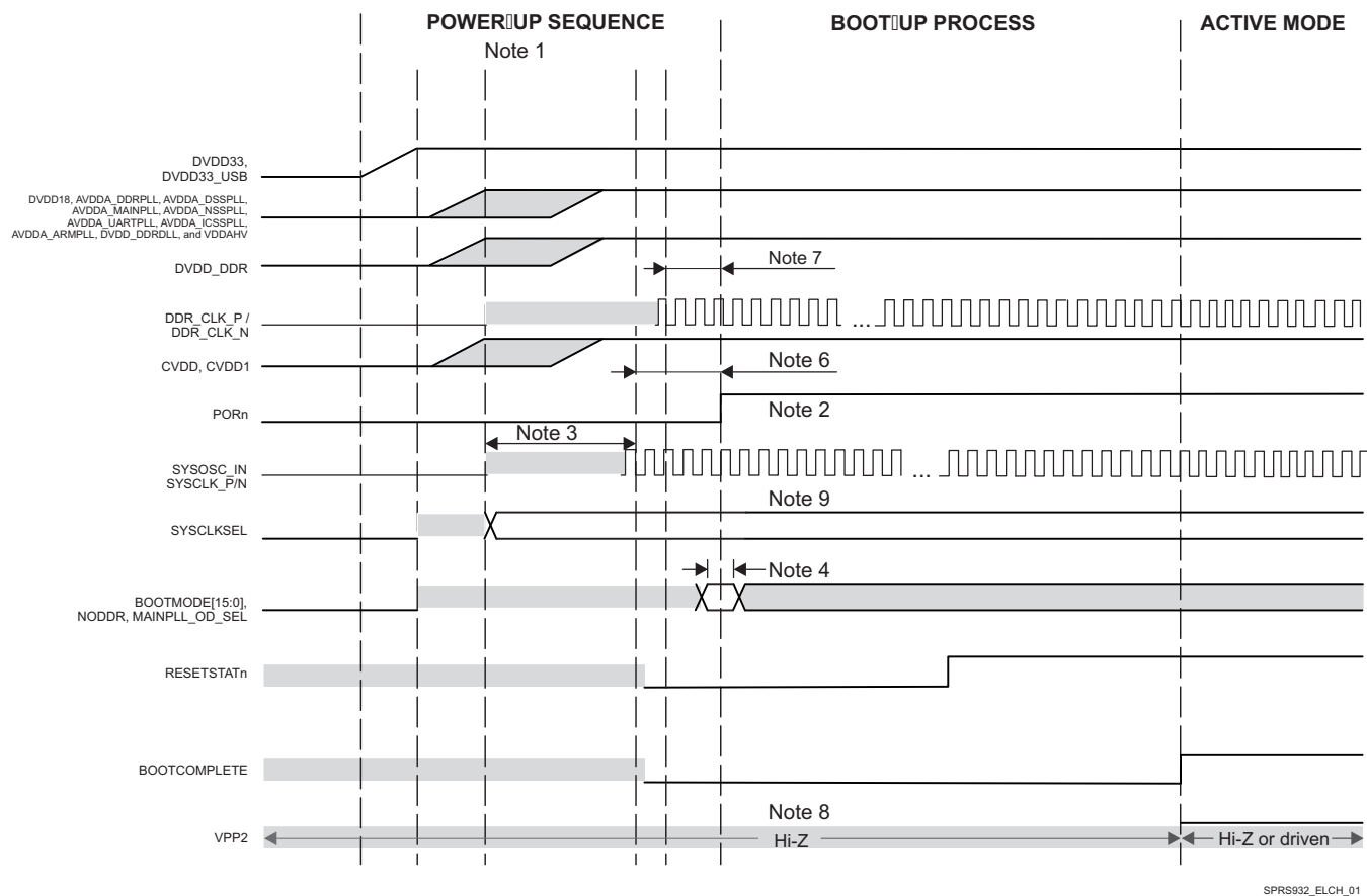
Figure 5-3. Power-Up Sequencing
