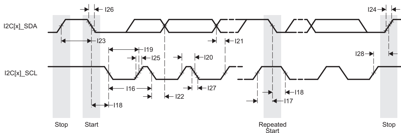
Figure 5-44. I2C Transmit Timing (1)
