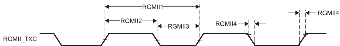
Figure 5-29. RGMII_TCX Timing - RGMII Mode
