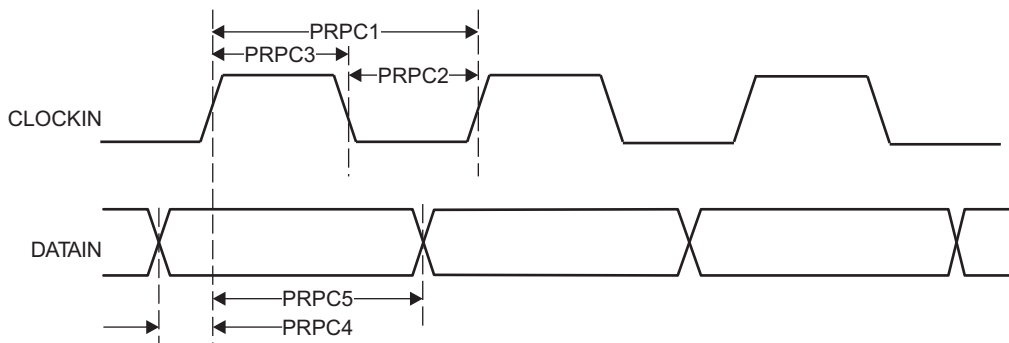
Figure 5-60. PRU-ICSS PRU Parallel Capture Timing – Rising Edge Mode
