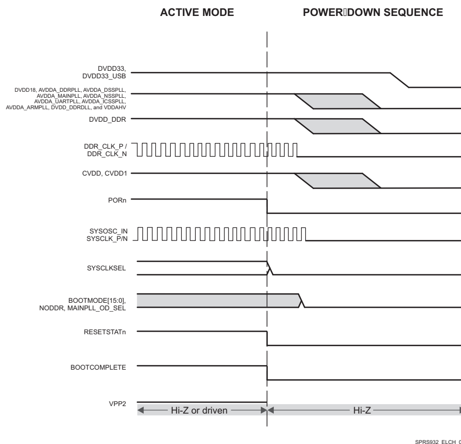
Figure 5-4. Power-Down Sequencing
