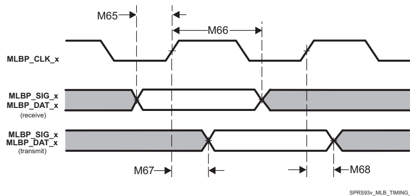
Figure 5-52. MLB 6-Pin Timing (1)
