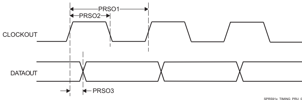
Figure 5-63. PRU-ICSS PRU Shift Out Timing
