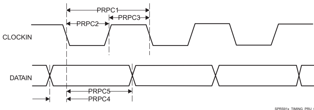
Figure 5-61. PRU-ICSS PRU Parallel Capture Timing – Falling Edge Mode
