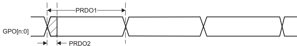
Figure 5-59. PRU-ICSS PRU Direct Output Timing
