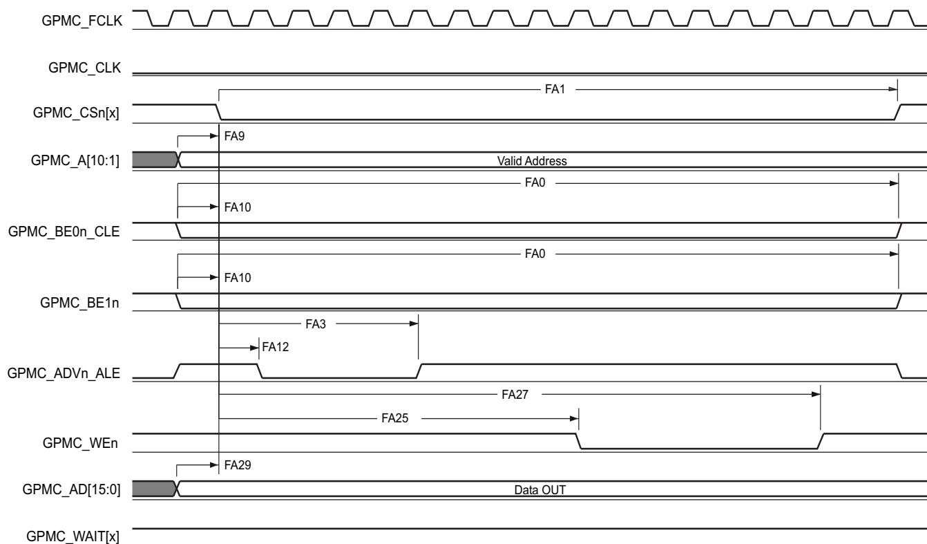
Figure 5-40. GPMC and NOR Flash—Asynchronous Write—Single Word
