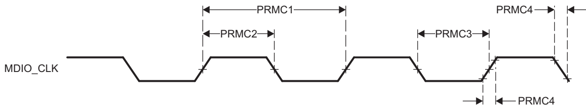
Figure 5-68. PRU-ICSS MDIO_CLK Timing
