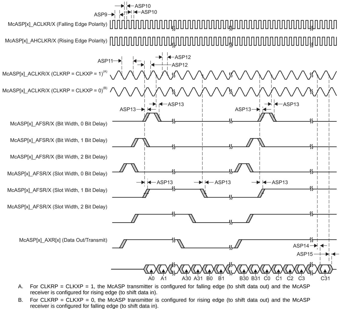
Figure 5-46. McASP Output Timing
