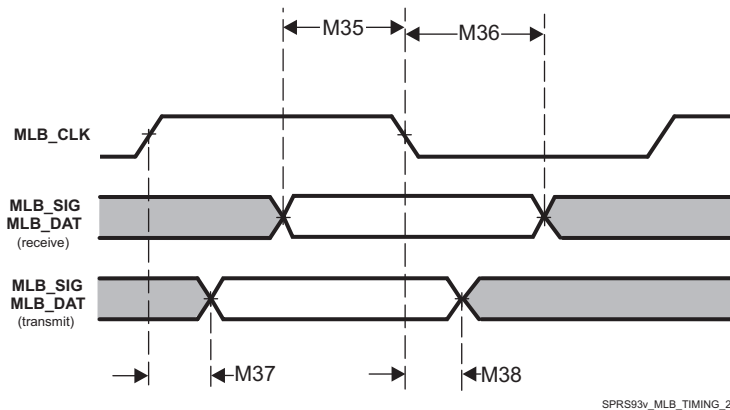
Figure 5-50. MLB 3-Pin Timing
