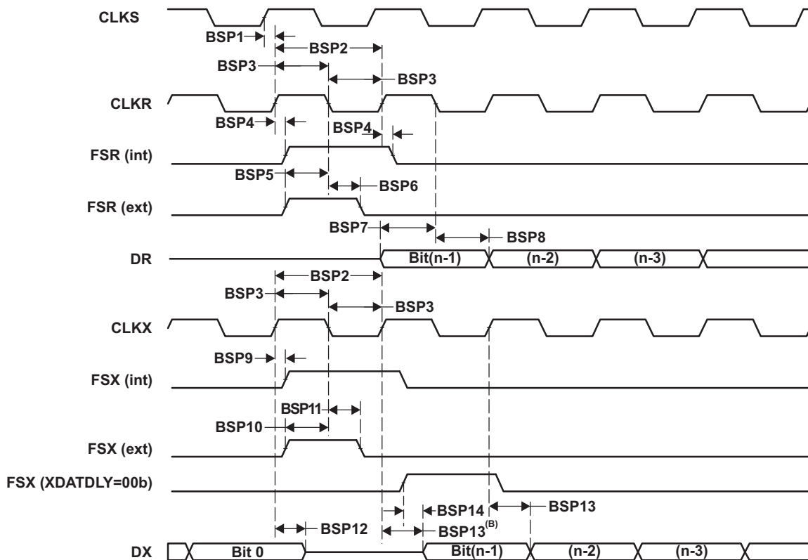
Figure 5-47. McBSP Timing
