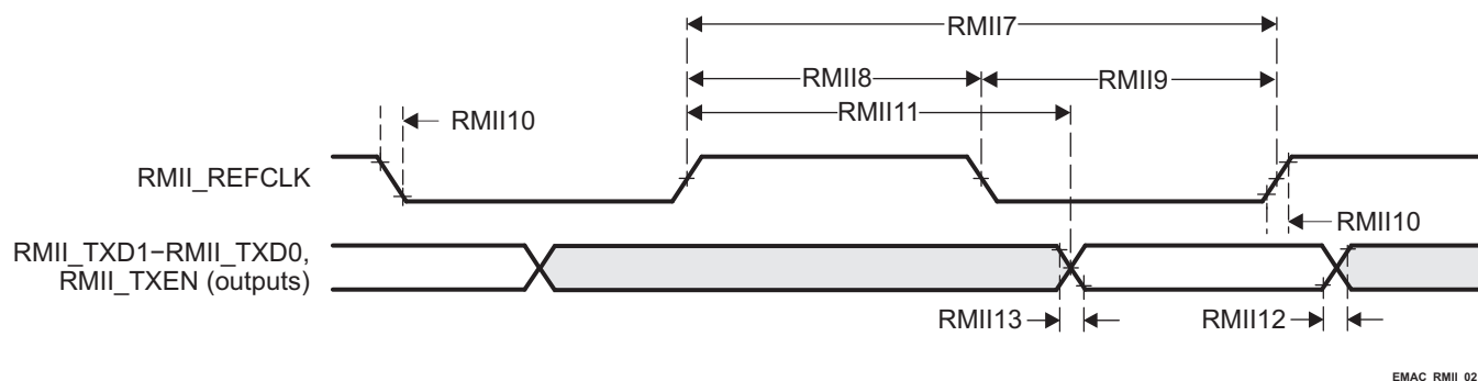
Figure 5-27. EMAC Transmit Interface Timing RMI Operation
