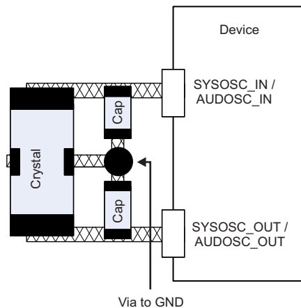
Figure 7-24. SYSOSC and AUDIOOSC PCB requirements
