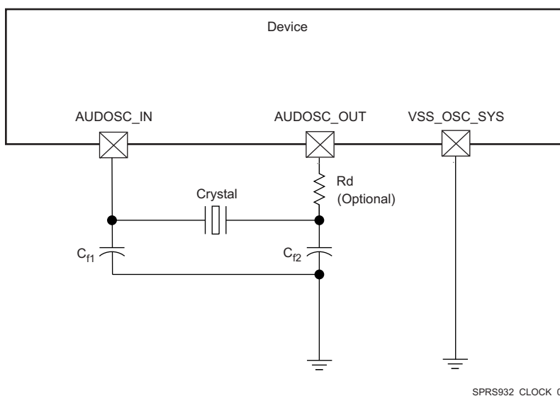
Figure 5-15. Crystal Implementation (1)
