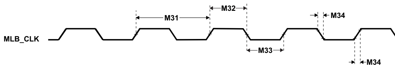
Figure 5-49. MLB_CLK Timing
