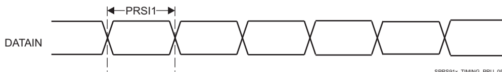
Figure 5-62. PRU-ICSS PRU Shift In Timing
