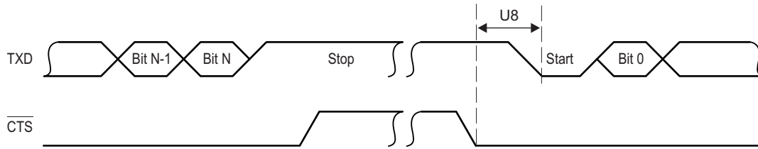
Figure 5-88. UART CTS (CTS to TXD Start Output) – Autoflow Timing Waveform
