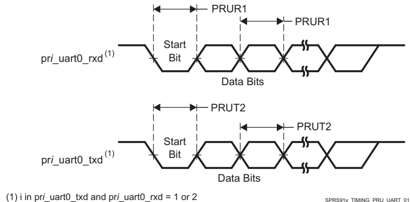
Figure 5-74. PRU-ICSS UART Timing
