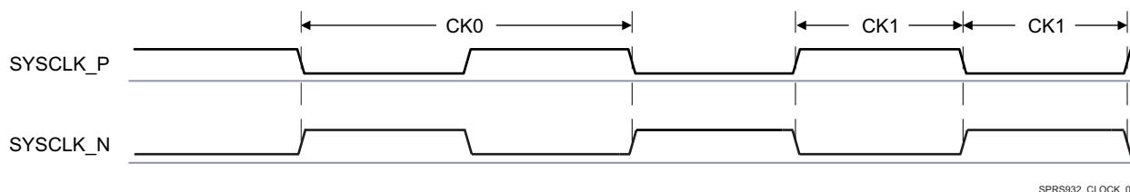
Figure 5-14. SYSCLK_P/N Input Clock
