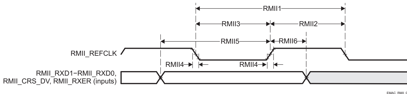
Figure 5-26. EMAC Receive Interface Timing RMI operation
