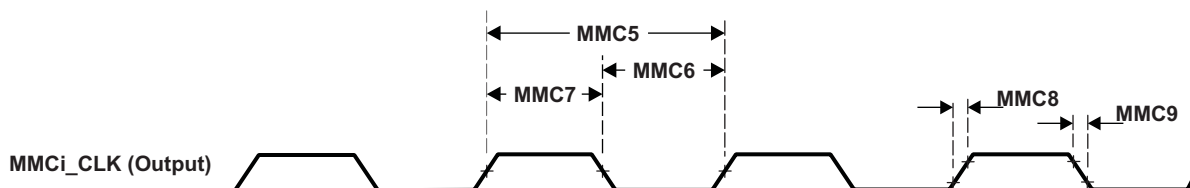
Figure 5-55. MMCi_CLK Timing (1)
