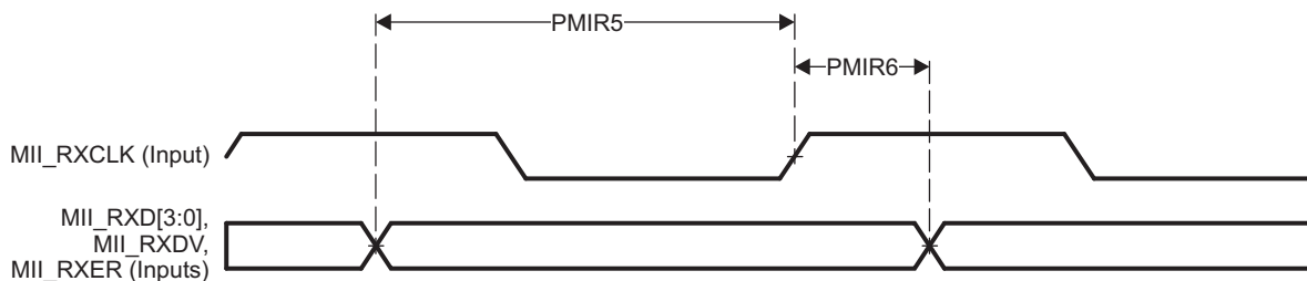
Figure 5-72. PRU-ICSS MII_RXD[3:0], MII_RXDV, and MII_RXER Timing
