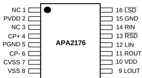
TSSOP-16 (Top View)
