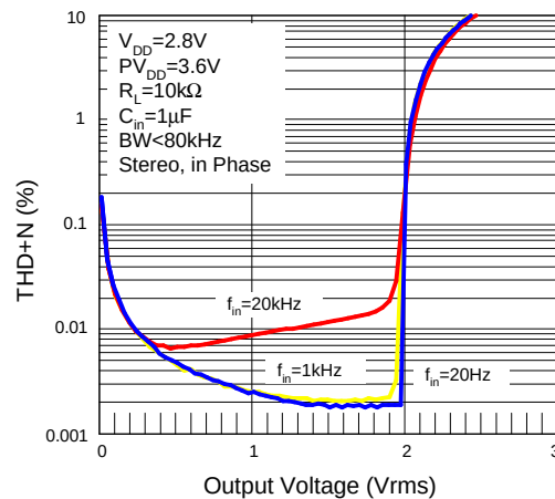
THD+N vs. Voltage
