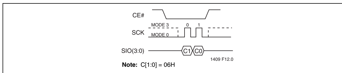
Figure 21:Write-Enable Sequence
