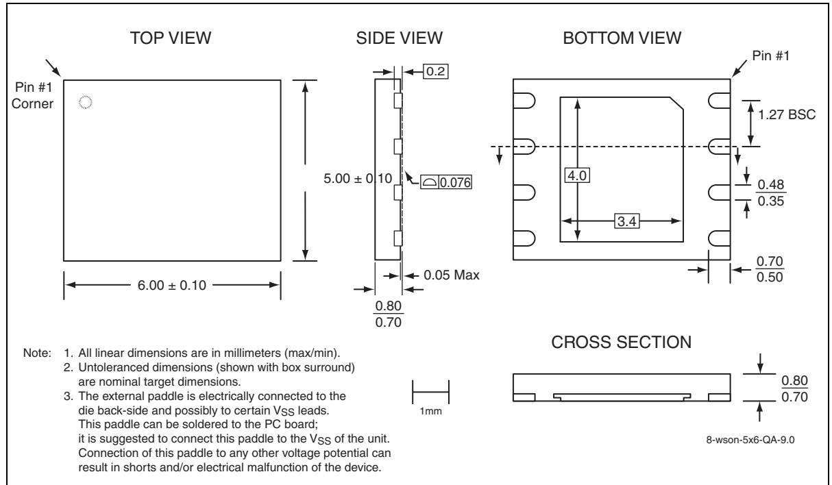
Figure 31: 8-Contact Very-very-thin, Small-outline, No-lead (WSO) SST Package Code: QA
