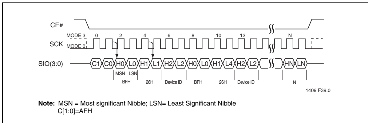
Figure 14: Quad J-ID Read Sequence
