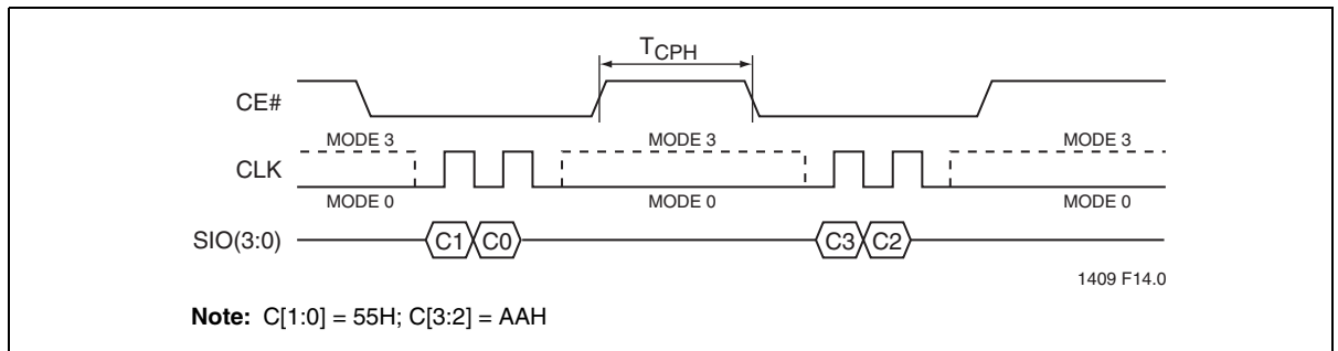
Figure 29: Reset Timing Diagram
