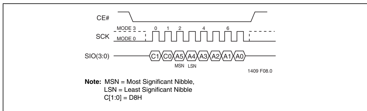
Figure 16:Block-Erase Sequence
