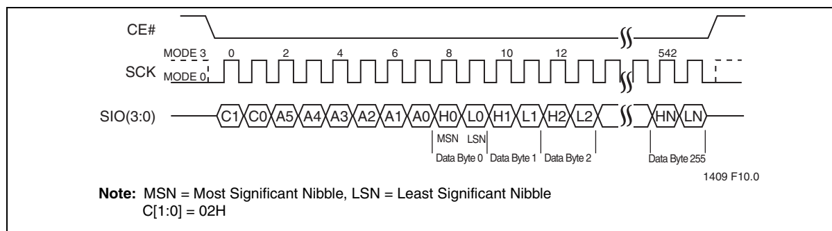
Figure 18: Page-Program Sequence
