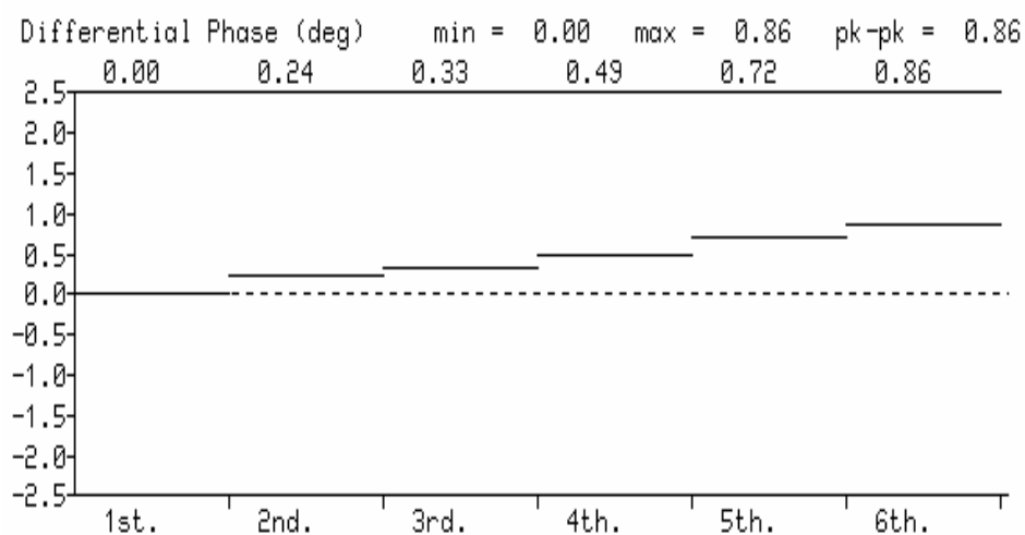
Figure 12. Differential Phase
