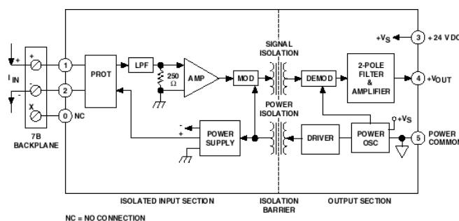
Figure 1. 7B35 Functional Block Diagram
