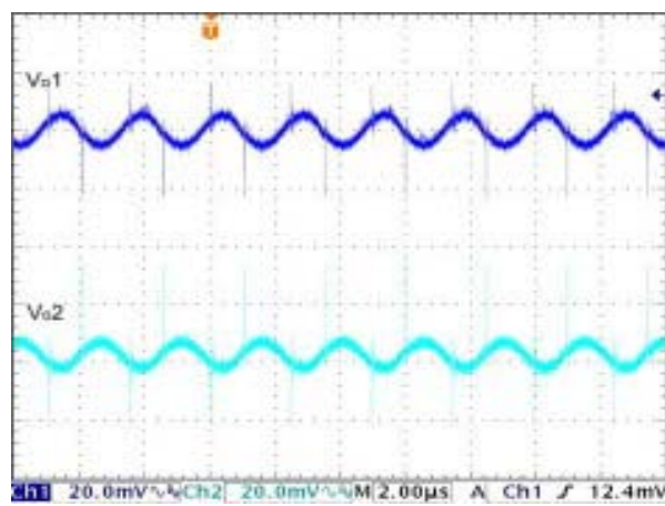
Graph 6: Typical Output Ripple and Noise (Nominal Vin and Full Load)
