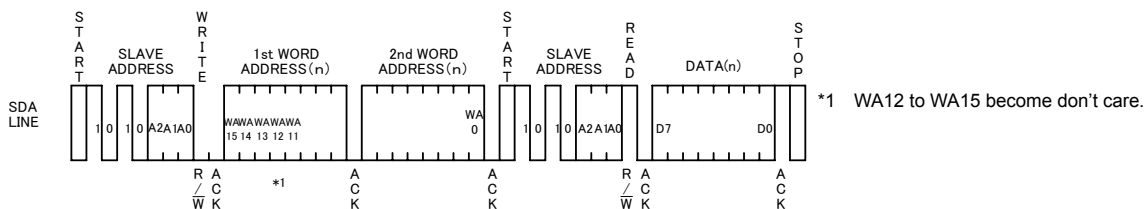
Fig.38 Random read cycle
