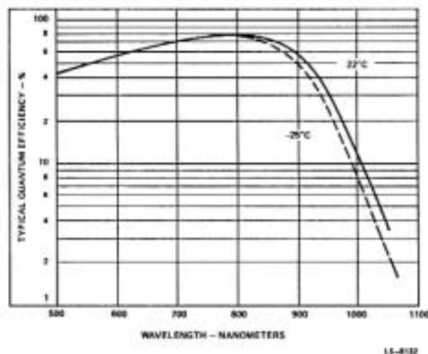
Figure 2. Typical Quantum Efficiency vs. Wavelength
