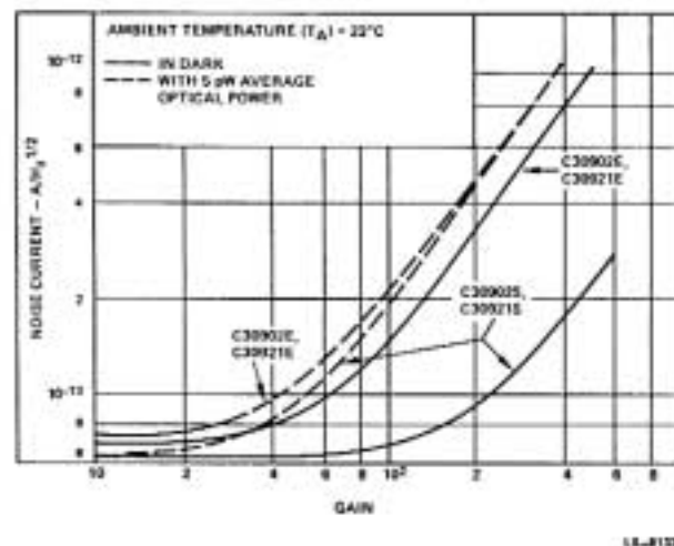
Figure 3. Typical Noise Current vs. Gain
