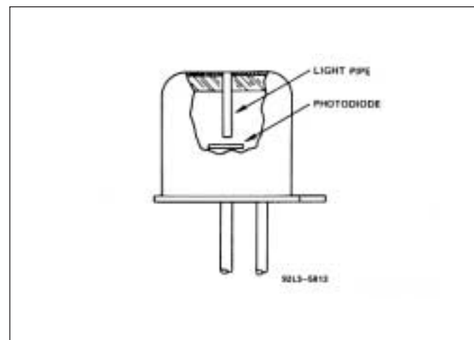
Figure 14. Cutaway of the C30921E, C30921S
