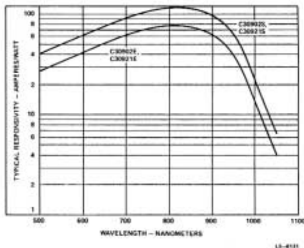
Figure 1. Typical Spectral Responsivity at 22°C
