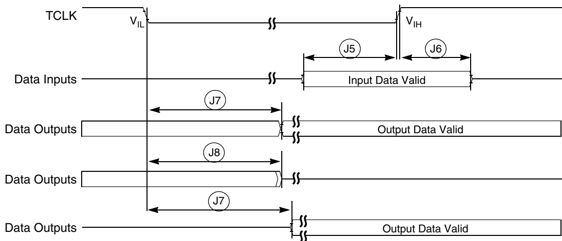
Figure 21. Boundary Scan (JTAG) Timing
