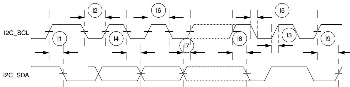
Figure 14. I²C Input/Output Timings
