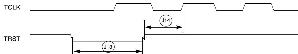
Figure 23. TRST Timing
