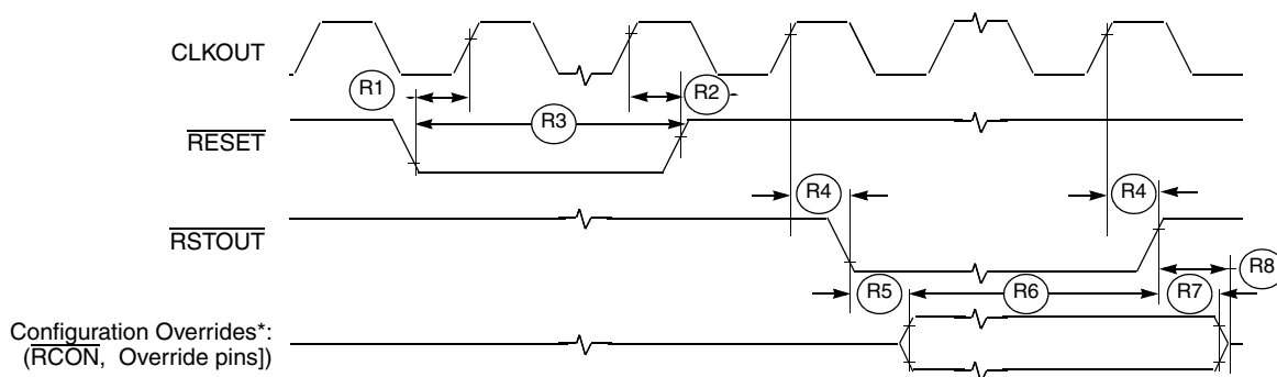
Figure 13. \overline{\text{RESET}} and Configuration Override Timing
