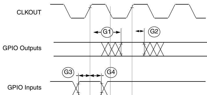
Figure 12. GPIO Timing
