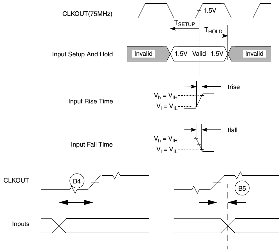
Figure 6. General Input Timing Requirements
