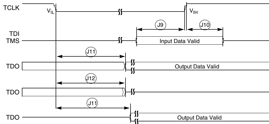
Figure 22. Test Access Port Timing
