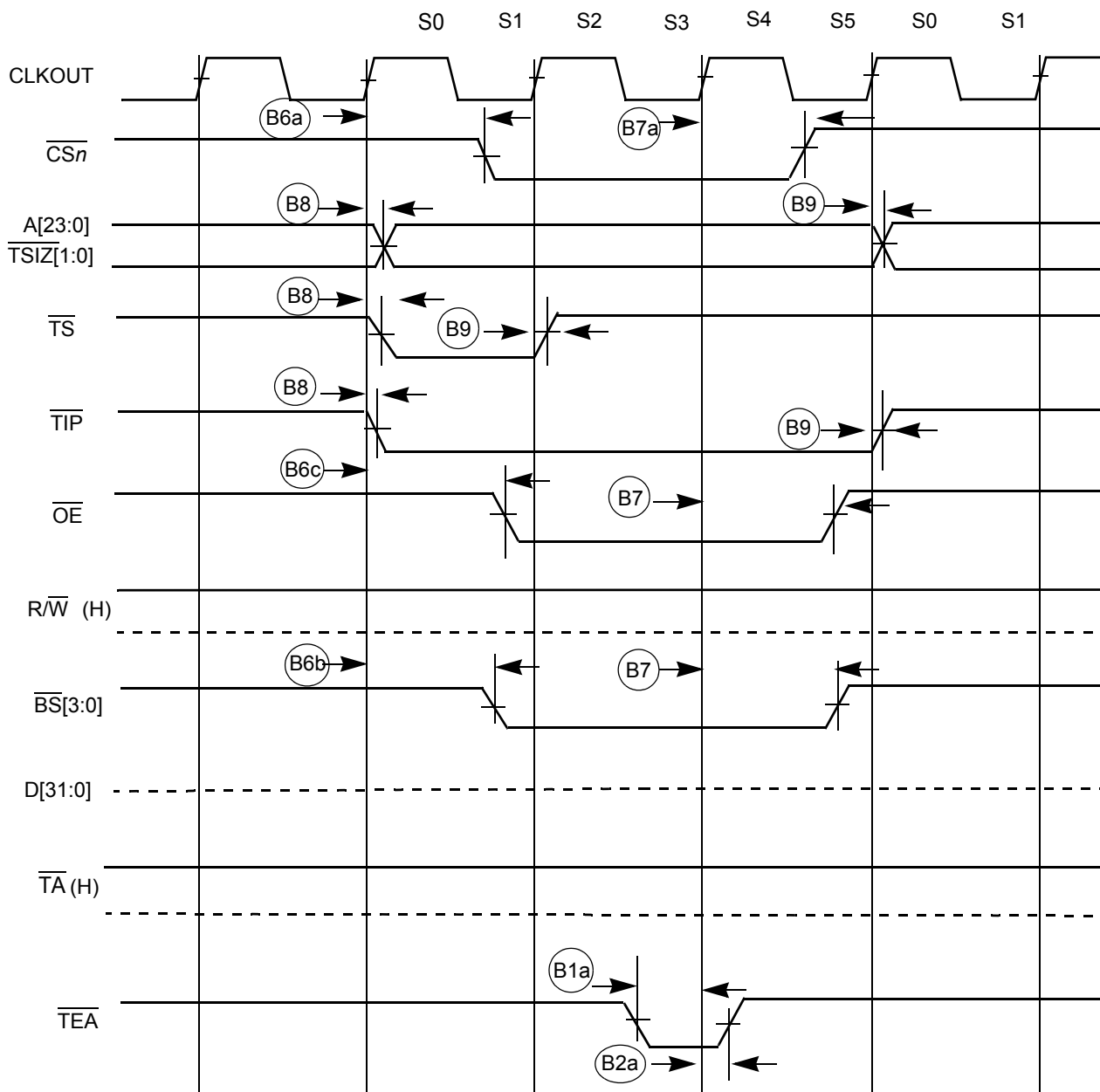
Figure 9. SRAM Read Bus Cycle Terminated by \overline{\text{TEA}}
