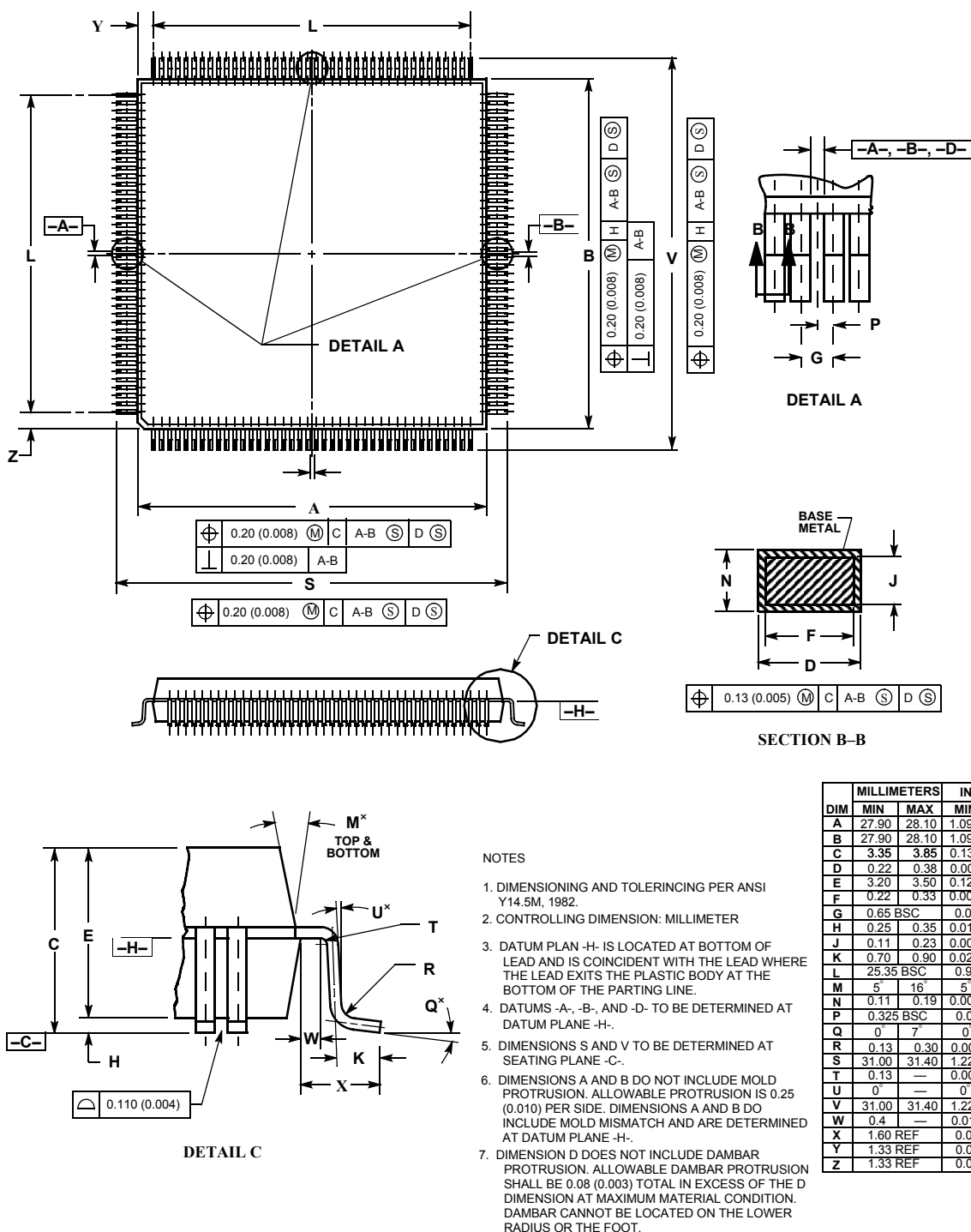
Figure 5. 160 QFP Package Dimensions
