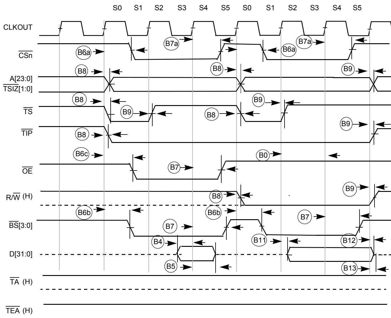
Figure 7. Read/Write (Internally Terminated) SRAM Bus Timing
