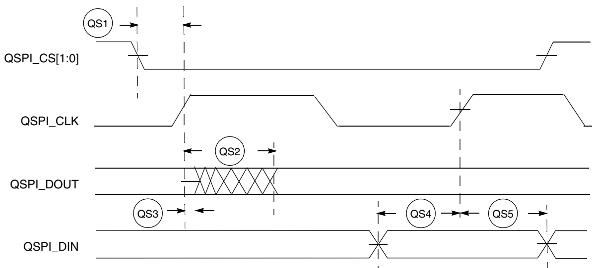
Figure 19. QSPI Timing
