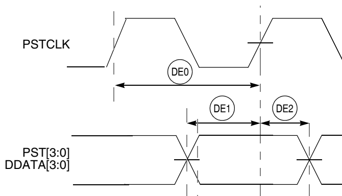
Figure 24. Real-Time Trace AC Timing
