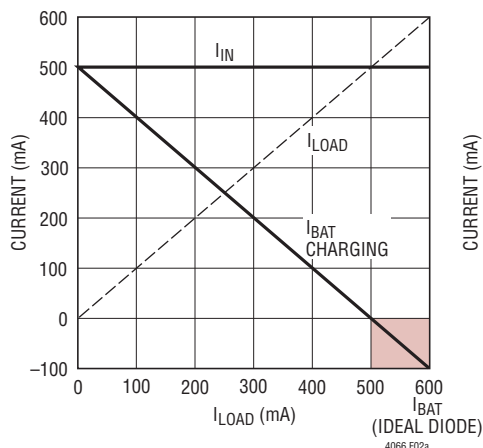
(2a) High Power Mode/Full Charge R_{PROG} = 100k and R_{CLPROG} = 2k
