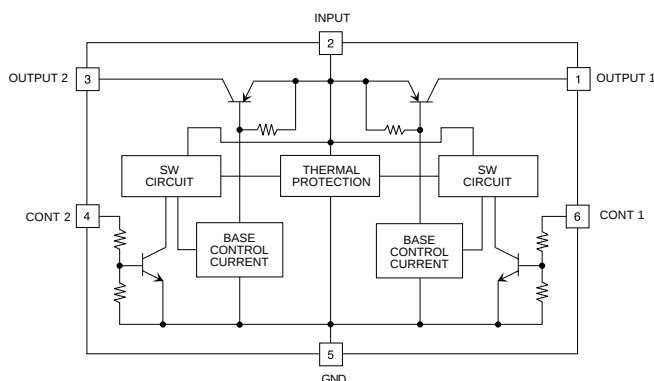
BLOCK DIAGRAM
