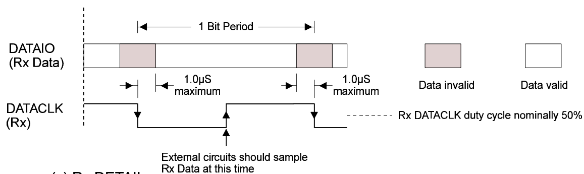
(c) Rx DETAIL
