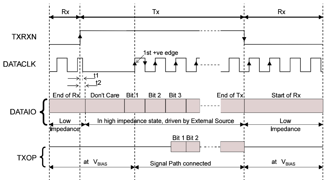
(a) DATA and CLOCK TIMINGS
