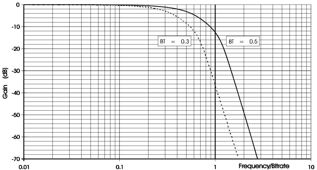
Figure 4 Typical Attenuation v. Frequency Response of Tx Filter (after external RC network)
