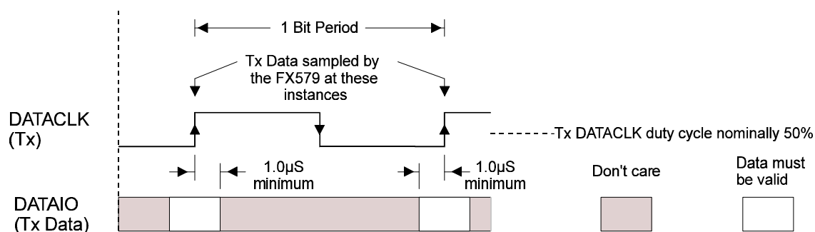
(b) Tx DETAIL
